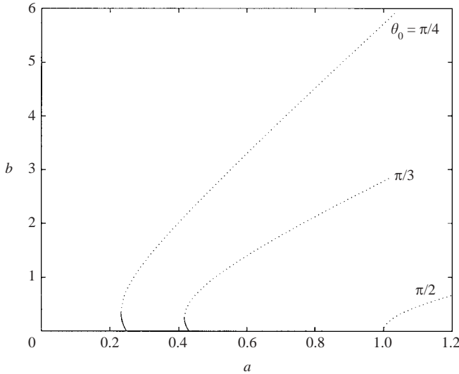
FIGURE 2. Solutions for b as a function of a with N=2 and the three choices of \theta_0 = \pi/2, \pi/3, \pi/4 . Note that in the case \theta_0 = \pi/2 there is only one solution for each a . The solid line denotes the solution for b corresponding to the negative-square-root branch in (8.11), the dotted line to the positive-square-root branch. The two solutions join smoothly when a = a_{crit} forming a continuous branch of solutions.
