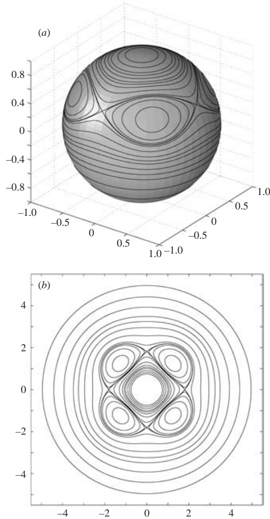
FIGURE 6. Solution for N=4 , a=0.15 and \theta_0=\pi/3 shown in orthographic (a) and stereographic projection (b). The corresponding values of b and \Omega_{max} are 0.81 and -92.74 respectively. There are point vortices, each of circulation 6\pi , at both the north and south poles.
