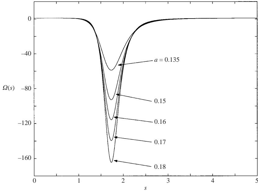
FIGURE 7. Graph of \Omega(s) against s for N=4 , \theta_0=\pi/3 and a=0.135, 0.15, 0.16, 0.17 and 0.18 . The respective values of \Omega_{max} are -58.77, -92.74, -115.70, -139.56 and -164.53 . As a increases, the vorticity profiles become more concentrated about the extremal value \Omega_{max} which itself increases in magnitude with increasing a .
