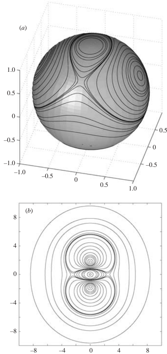
FIGURE 4. Solution for N=2 , a=1 and \theta_0=\pi/3 shown in orthographic (a) and stereographic projection (b). The corresponding values of b and \Omega_{max} are 2.78 and -173.93 respectively. There are point vortices, each of circulation 2\pi , at both the north and south poles.
