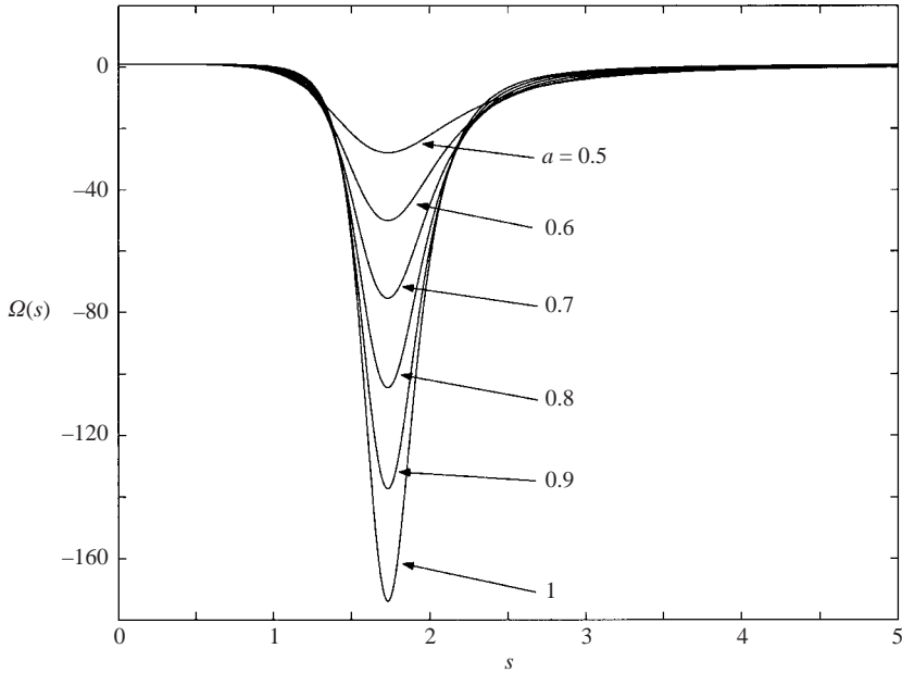
FIGURE 5. Graph of \Omega(s) against s for N=2 , \theta_0 = \pi/3 and a = 0.5, (0.1), 1 . The respective values of \Omega_{max} are -27.93, -50.09, -75.51, -104.55, -137.35 and -173.93 . As a increases, the vorticity profiles become more concentrated about the extremal value \Omega_{max} which itself increases in magnitude with increasing a .
