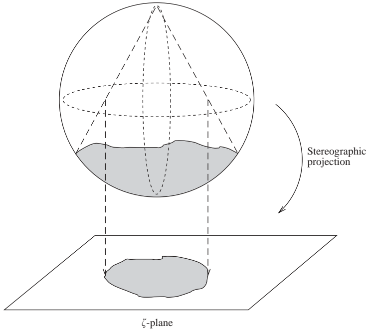
FIGURE 1. Schematic illustrating stereographic projection from the sphere to a complex \zeta -plane.
