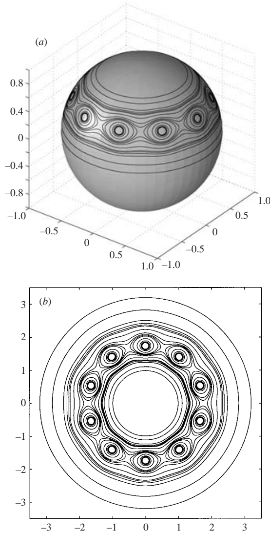
FIGURE 8. A row of 10 Stuart vortices at latitude \pi/3 shown in orthographic (a) and stereographic projection (b). The solution parameters are N=10 , a=0.01 , b=2.203 and \theta_0=\pi/3 . There are point vortices, each of circulation 18\pi , at both the north and south poles.
