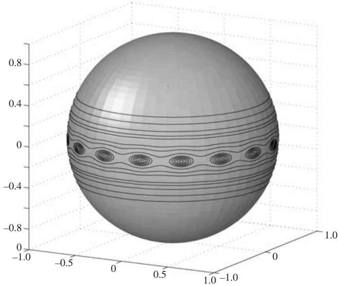
FIGURE 9. A row of 16 Stuart vortices at the equator. The solution parameters are N = 16 , a = 1.05 , b = 0.320 and \theta_0 = \pi/2 . There are point vortices, each of circulation 30\pi , at both the north and south poles.
