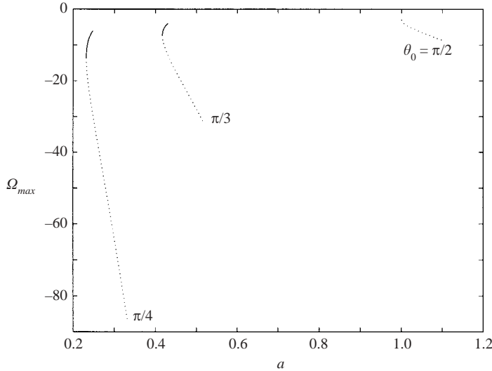
FIGURE 3. \Omega_{max} as a function of a with N=2 and the three choices of \theta_0 = \pi/2, \pi/3, \pi/4 . The solid line denotes the value of \Omega_{max} derived using the solution for b corresponding to the negative-square-root branch in (8.11), the dotted line to that computed using the positive-square-root branch.
